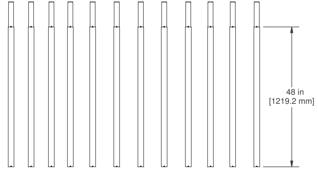
QTY. (12) CF TUBE SECTION P/N: 4112201
