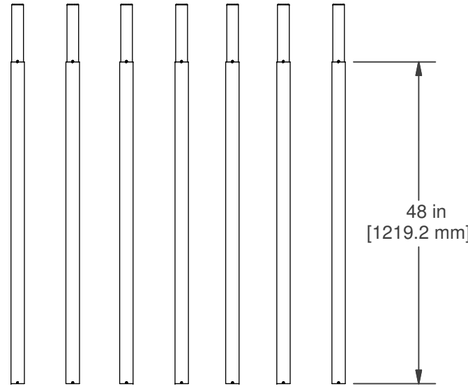
QTY. (7) CF TUBE SECTION P/N: 4112201
