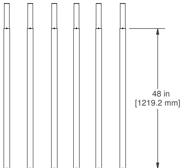
QTY. (6) CF TUBE SECTION P/N: 4112201
