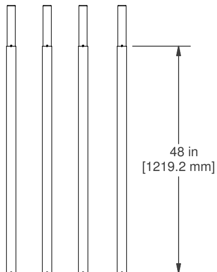
QTY. (4) CF TUBE SECTION P/N: 4112201
