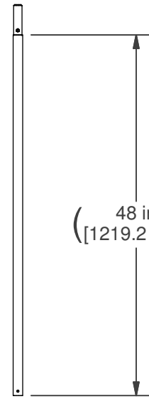
48 in [1219.2 mm] QT'Y. (1) TUBE SECTION P/N: 4132801
