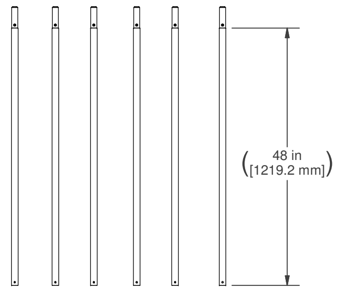
QT'Y. (6) TUBE SECTION P/N: 4120601
