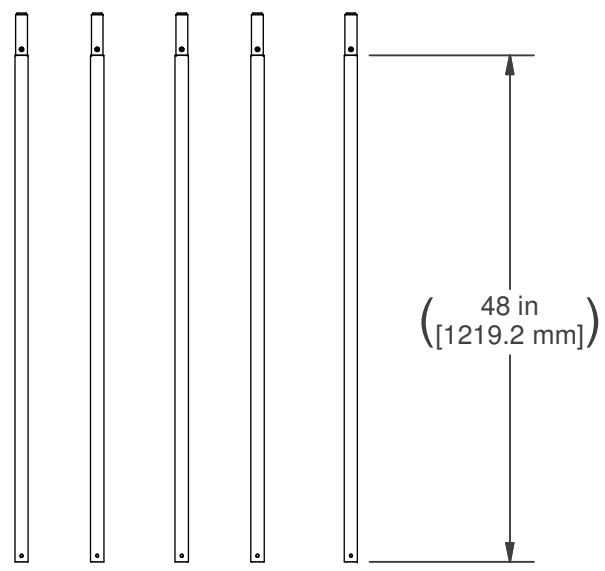
QTY. (5) TUBE SECTION P/N: 4120601
