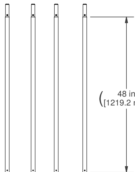
QT'Y. (4) TUBE SECTION P/N: 4120601
