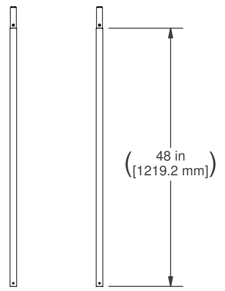
QTY. (2) TUBE SECTION P/N: 4120601
