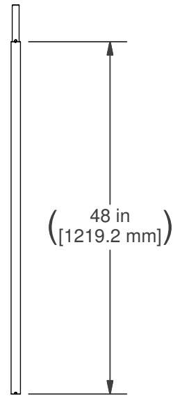
QTY. (1) TUBE SECTION P/N: 4132801
