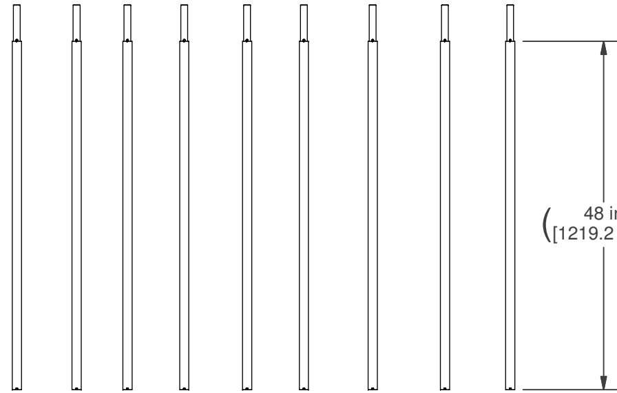
QTY. (9) TUBE SECTION P/N: 4132801
