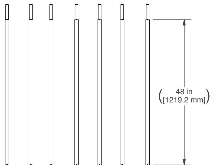
QT'Y. (7) CF TUBE SECTION P/N: 4132801
