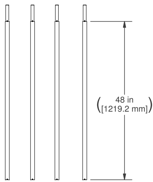
QT'Y. (4) CF TUBE SECTION P/N: 4132801
